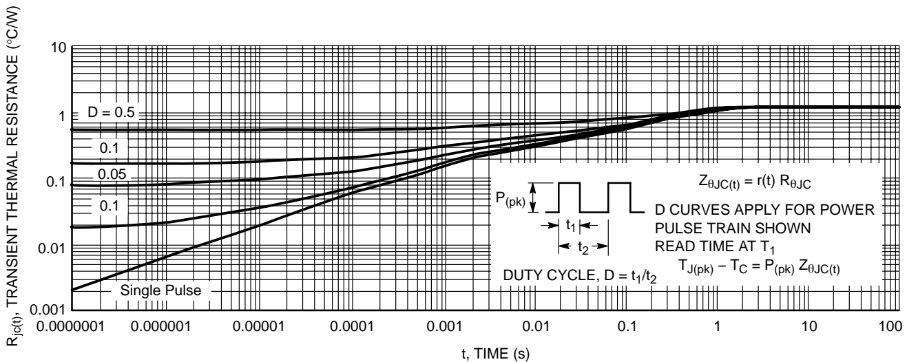
Figure 9. Thermal Response
